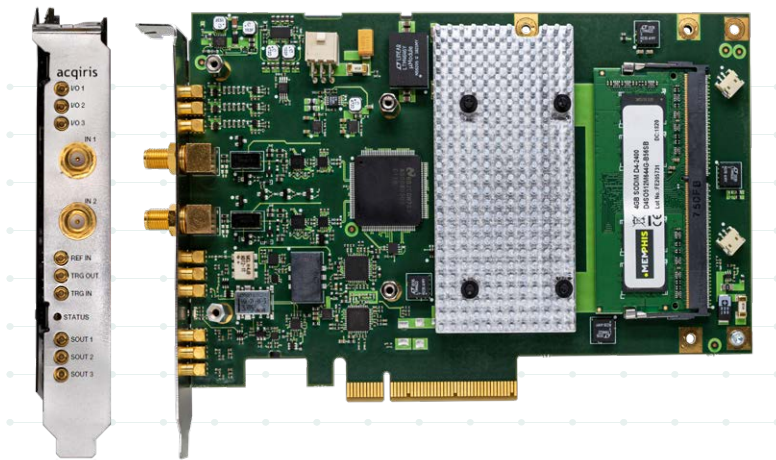
Figure 2. SA1 ADC card - Front panel, with analog inputs, multiple programmable I/O signals and unique synchronized I/Os. Open view.
