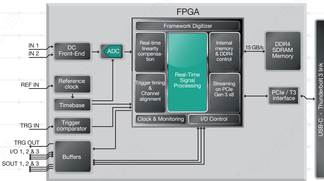
Figure 3. Top level block diagram of the SA120E ADC module, with on-board real-time processing.
